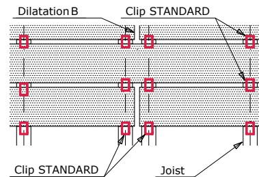
Pic. 5 - Butting deck boards with STANDARD clip.
